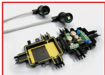
P111401 00001 - VENTIMIGLIA NS Infrared obstacle detection device for BIR C safety edge compliant with standard EN 12978.
